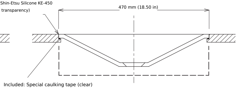
B-B' Section
